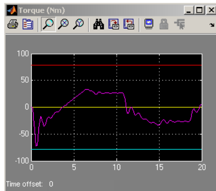
Servomechanism Simulation Scopes
