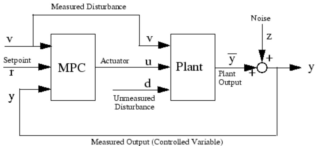
Block Diagram of a SISO Model Predictive Control Toolbox™ Application
