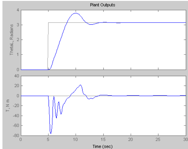
Servo Response for Step Increase of \pi Radians
